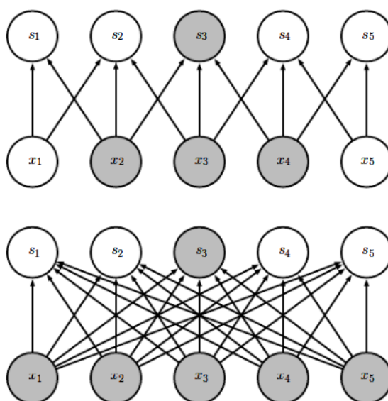
Figure 4.5: Sparse connectivity.
