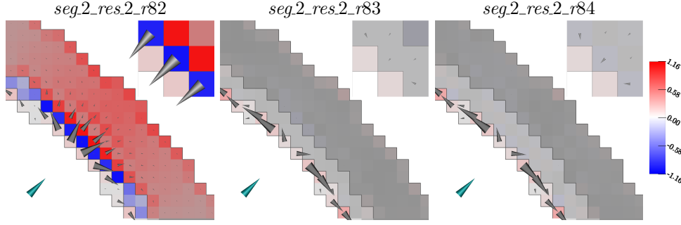
FIG. 10. Visualization of current flow differences between the CG-FEM and DG-FEM in models seg2_res2_r82 (left), seg2_res2_r83 (middle), and seg2_res2_r84 (right). The turquoise cone presents the dipole source. The coloring shows the \ln \text{MAG}_{j,\text{loc}} (increase/decrease of the current strength simulated with the CG-FEM compared to the DG-FEM solution). For all models the maximum of the color scale is chosen as the maximal value in the skin and skull compartment. Gray cones, having the same linear scaling for all models, show the \text{totDIFF}_{j,\text{loc}} (difference in current flow). In models seg2_res2_r83 and seg2_res2_r84 , the arrows in skin and skull are not visible due to the relatively small values. Dark gray lines mark compartment boundaries. In the top right corner of each subfigure, a detail of the skull elements to which the dipole is pointing is shown. The size of the cones is magnified by a factor of 20 compared to the full image, and only the cones for the skull compartment are visualized.
