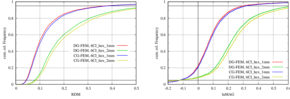
FIG. 11. Cumulative relative errors of the RDM (left) and lnMAG (right) in realistic six-layer hexahedral head models with 1- and 2-mm mesh resolutions in reference to high-resolution tetrahedral model.
