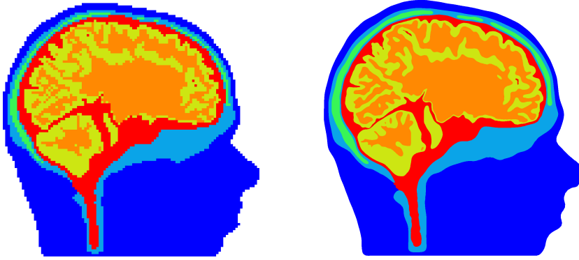
FIG. 5. Visualization of realistic six-compartment hexahedral 6CL_{\text{hex}_2\text{mm}} , h = 2\text{mm} , (left) and high-resolution reference head model 6CL_{\text{tet\_hr}} (right).
