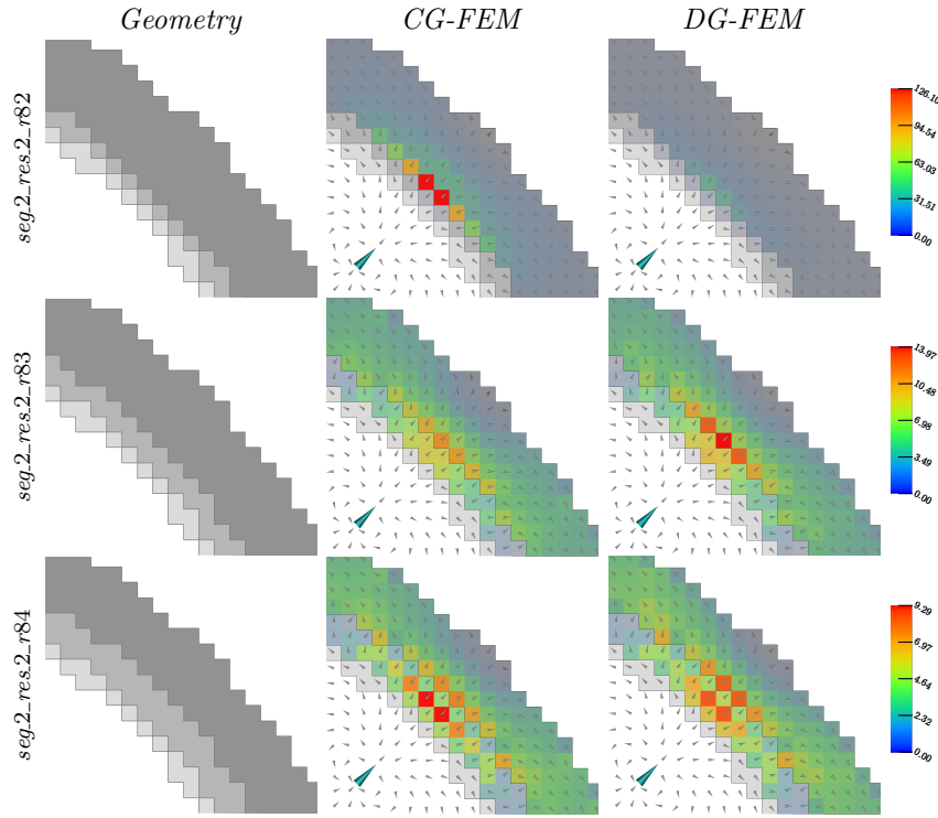
FIG. 9. Visualization of model geometry (left column), current direction and strength for the CG-FEM (middle column) and DG-FEM (right column) for models seg.2_res.2_r82 (top row), seg.2_res.2_r83 (middle row), and seg.2_res.2_r84 (bottom row). The left column shows the model geometry, interior to exterior from bottom left to top right, brain in white, CSF, skull and skin in increasingly dark gray, and air in white. Dark gray lines mark compartment boundaries. In the middle and right columns, the large turquoise cone presents the dipole source. The small and normalized gray cones show the directions of the current flow and, for elements belonging to skull and skin compartments, the coloring indicates the current strength. For each model, the color scale is kept constant for both approaches.
