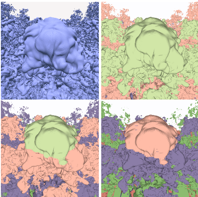
Fig. 12. Qualitative impact of multiresolution on the Richtmyer-Meshkov data at t=270 , isovalue 20. Top left to bottom right: single-ray, then coherent multiresolution with dP/dV of 1.2 and 4. On an Intel Core Duo 2.16 GHz with a 512^2 frame buffer, these render at 0.92, 1.0, 1.9, and 3.6 FPS respectively. To illustrate LOD transitions, like colors indicate the same resolution.
