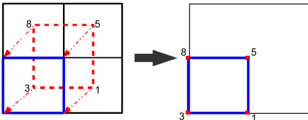
Fig. 2. Voxel-cell mapping. Given a scalar-centered voxel (blue outline), we construct a cell at that location by mapping the scalar to the lower-most vertex, and assigning forward neighboring scalars to the remaining vertices. This is equivalent to the dual, but spatially offset to align with the coordinate frame of the voxel.
