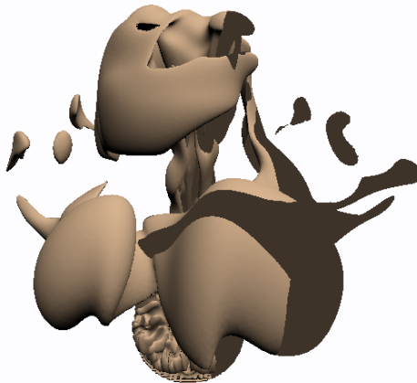
Fig. 11. Shadows. By coherently casting shadow rays through a coarser-resolution version of our data, we achieve higher performance while providing similar spatial depth cues as shadows cast on the full-resolution volume. With centrally-differenced gradient normals, the above shadowed scene renders at 3.9 FPS on an Intel Core Duo 2.16 GHz with a 512^2 framebuffer; only slightly slower than without shadows at 5.1 FPS.
