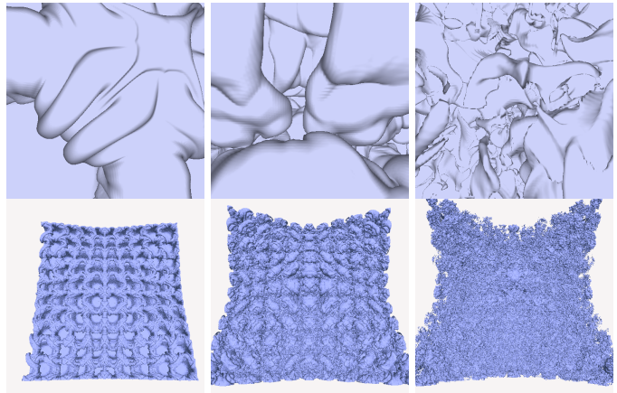
Fig. 13. Richtmyer-Meshkov results . From left to right, timesteps 50, 150 (isovalue 20), and 270 (isovalue 160). Top: various close-up camera views, illustrating highly coherent scenes. We use dP/dV = 1 . Bottom: far views with the same camera position, exhibiting generally poor coherence.
