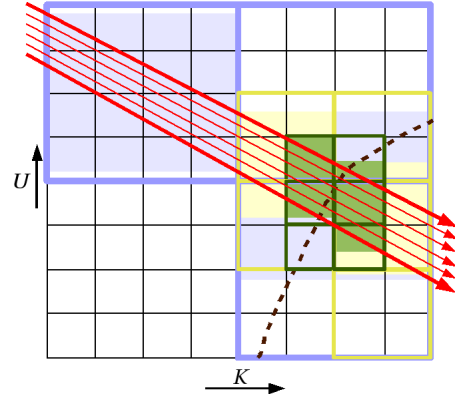
Fig. 5. Coherent Octree Traversal via Implicit Macrocells. Our hierarchical grid employs recursively superimposed macrocell blocks, with each parent containing 2^3 children, for alignment with the octree volume. We depict a 3-deep hierarchy, with blue, yellow and green extents corresponding to macrocell layers from coarsest to finest. Macrocells are only traversed when they contain our desired isovalue, as illustrated by the “surface” at the dotted line. With an octree, macrocells are implicit, and their min/max pairs are retrieved from the octree volume via hashing.
