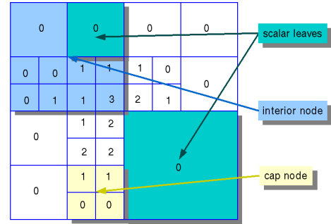
Fig. 1. Octree volume format illustrated, showing examples of an interior node, a cap node, and scalar leaves. A scalar leaf is not a separate structure, but rather a single value embedded inside its parent interior node. Similarly, cap nodes are not leaves themselves but contain eight scalars at the maximal depth of the octree. Thus, nodes in this structure are the parents of nodes in the logical octree.
