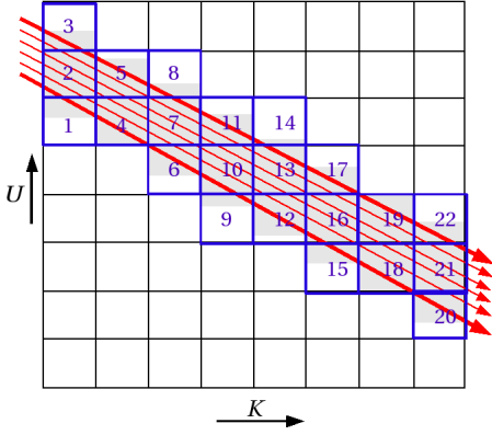
Fig. 4. Coherent Grid Traversal. The classic CGT algorithm traverses a packet of rays through a grid slice by slice along a major march axis \vec{K} , incrementing each subsequent slice extents by the differential of the bounding frustum along the non-major axis \vec{U} , as well as the third axis \vec{V} in the 3D case. This illustration numbers the grid cells in the order of their traversal. Unlike the single-ray DDA grid algorithm, cells may be traversed in arbitrary \vec{U}, \vec{V} order; however the \vec{K} order is invariably front to back.
