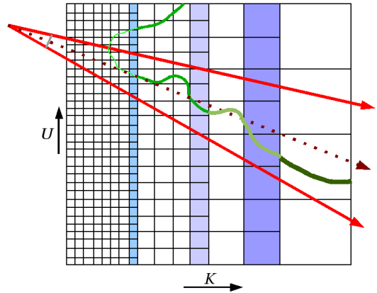
Fig. 8. Multiresolution transition slices . We determine transition slices along the major march axis \vec{K} , transitioning from finer to coarser resolution as slices progress from the camera origin. For the transitions, we determine the last k -slice where each resolution level corresponds to a fixed voxel-to-pixel ratio.
