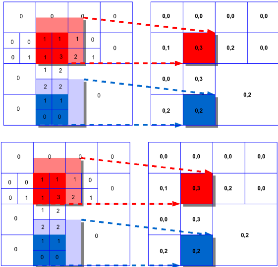
Fig. 3. Min/max tree construction from forward neighbors. Top: Each leaf node must compute the minimum and maximum of its cell, hence account for the values of neighbors in the positive X and Y dimensions (left). This yields a min/max pair for the leaf node (right). Neighbors can potentially exist at different depths of the octree, as is the case for at the blue leaf node. Bottom: For multiresolution data, we must include wider neighbors at coarser resolutions into the min/max computation.
