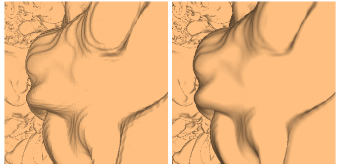
Fig. 10. Gradient normals, computed on a forward differences stencil yielding 5.5 FPS (left), and a central differences stencil at 4.7 FPS (right) on an Intel Core Duo 2.16 GHz with a 512^2 frame buffer. The lookup overhead of a 4^3 neighborhood of voxels makes central differences extremely costly in a single-ray or depth-first system. The slice-based coherent scheme delivers smooth normals with a far lesser penalty.
