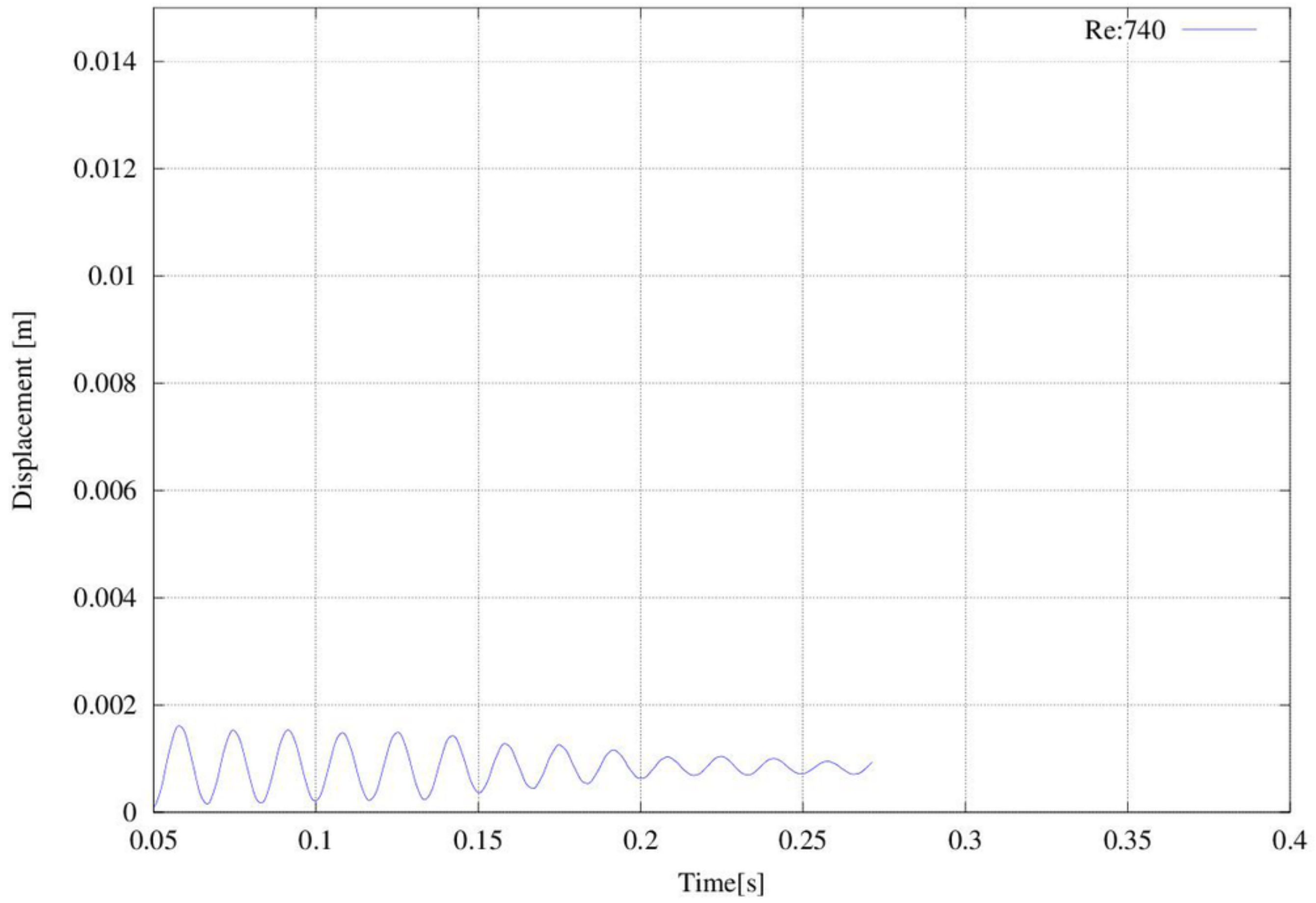
Scoping Run: Re:740 AR:10 Grid Resolution dx=dy=dz=D/8
