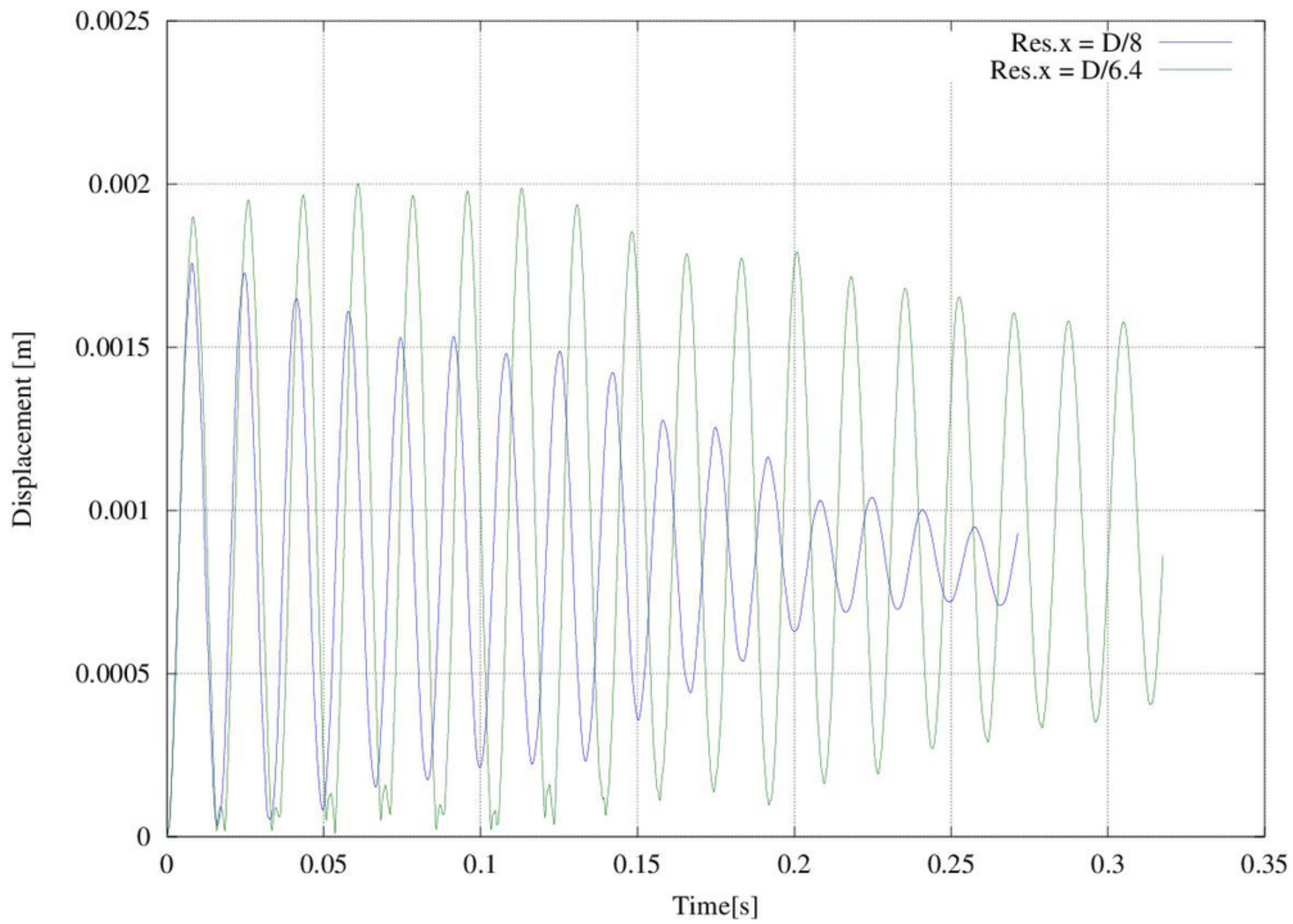
1 Pin Fin, Re:740, AR:10, Resolution Comparison
