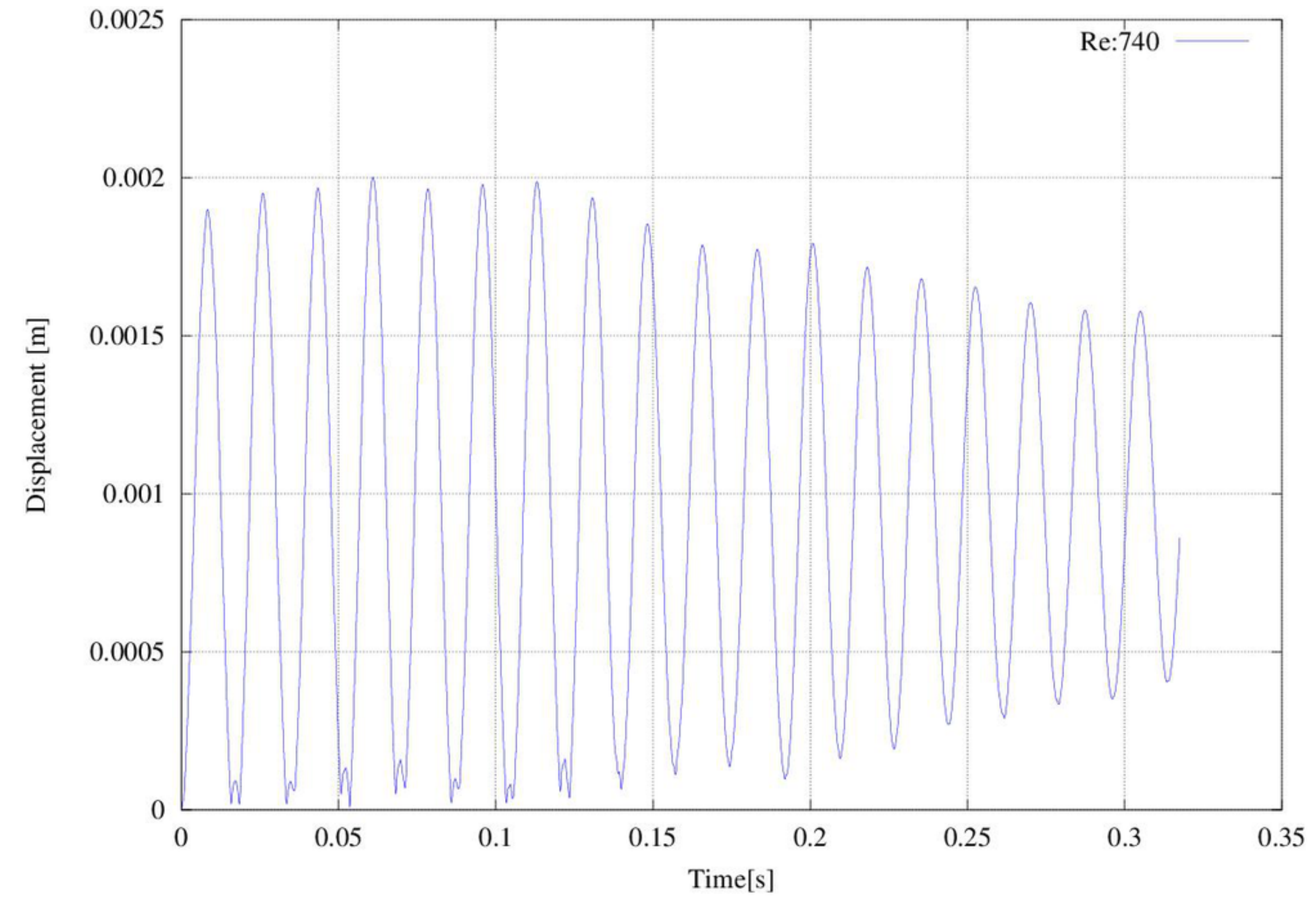
Scoping Run: Re:740 AR:10 Grid Resolution dx=dy=dz=D/8
