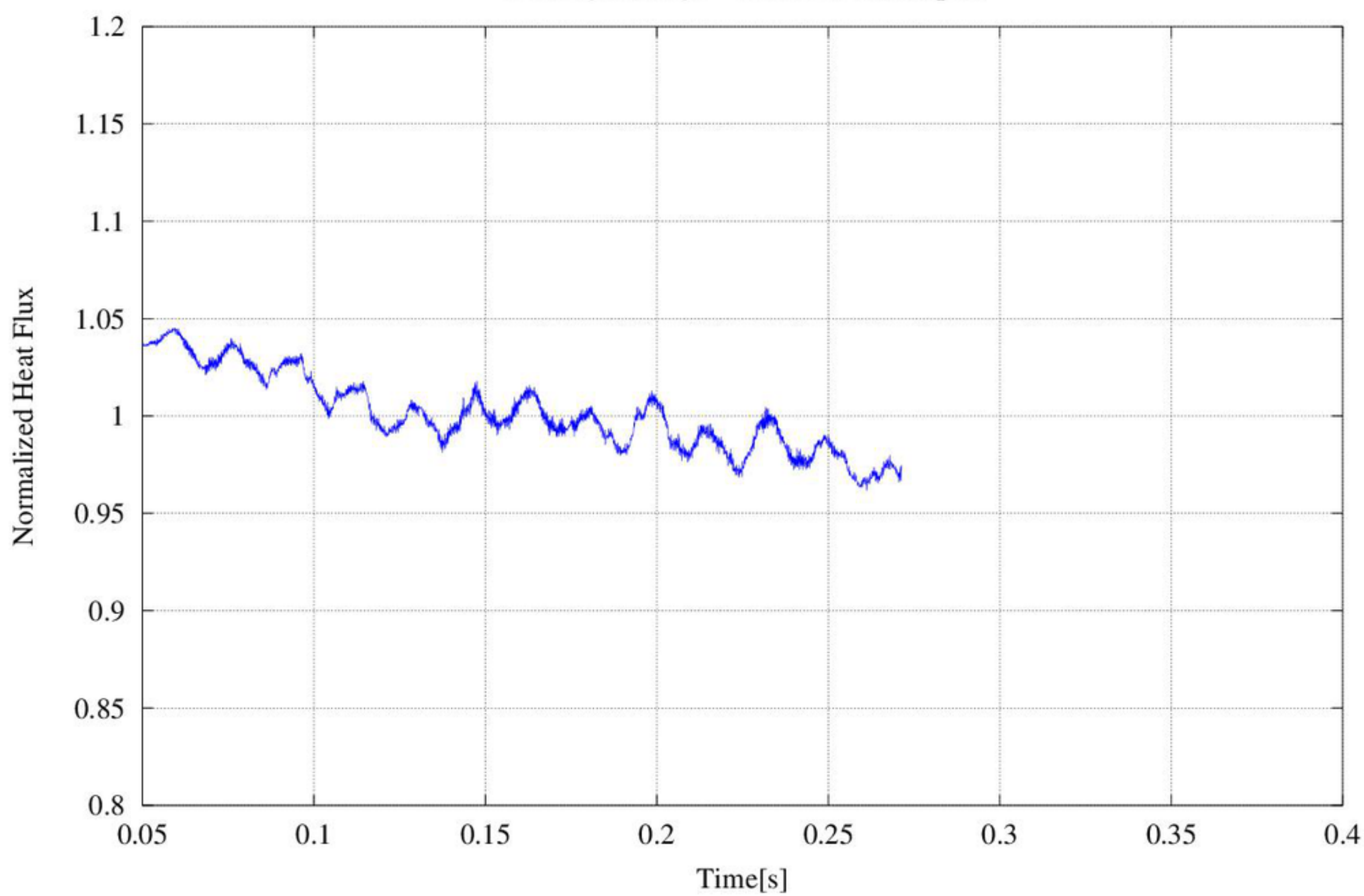
Flow Around One Flexible Cylinder, Wrong dx Re:740, AR:10 Heat flux: D/8 vs D/6.4 Moving Average = 0.01sec, 100 samples
