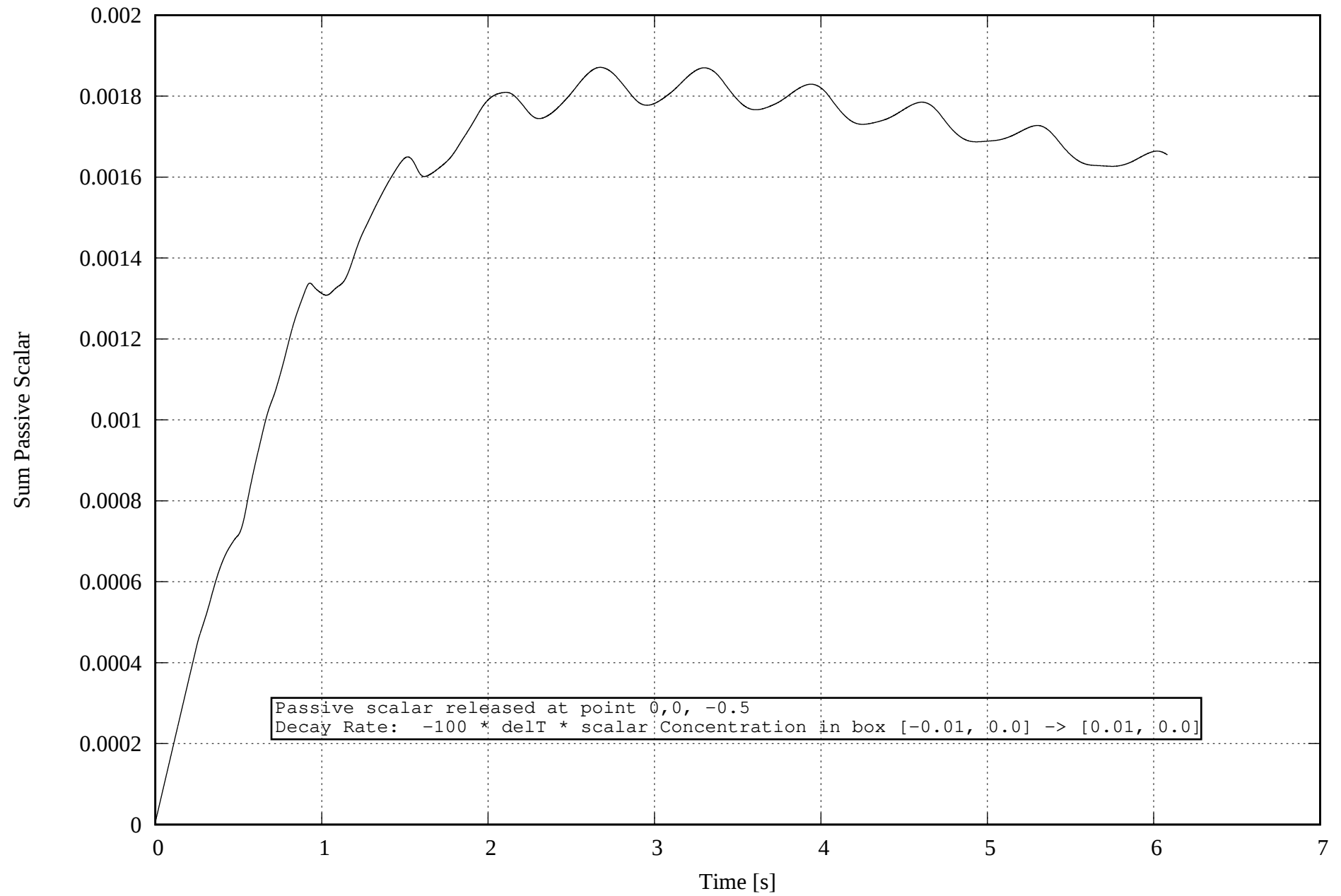
Passive Scalar Released in a Vortex
