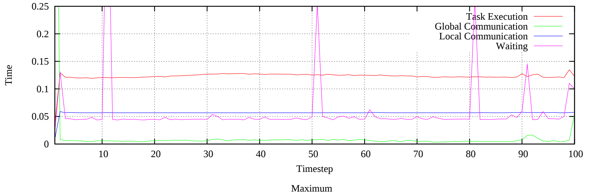
Explicit MPMICE: Thu Nov 8 2012 : c301-314.ls4.tacc.utexas.edu : 96 Processors Averaged over all processors
