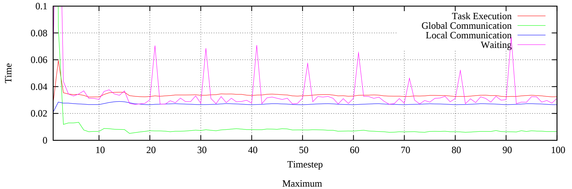
Explicit MPMICE: Thu Nov 8 2012 : c301-112.ls4.tacc.utexas.edu : 384 Processors Averaged over all processors
