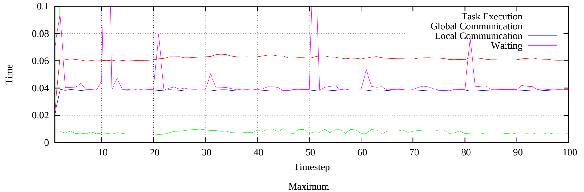
Explicit MPMICE: Thu Nov 8 2012 : c301-314.ls4.tacc.utexas.edu : 192 Processors Averaged over all processors
