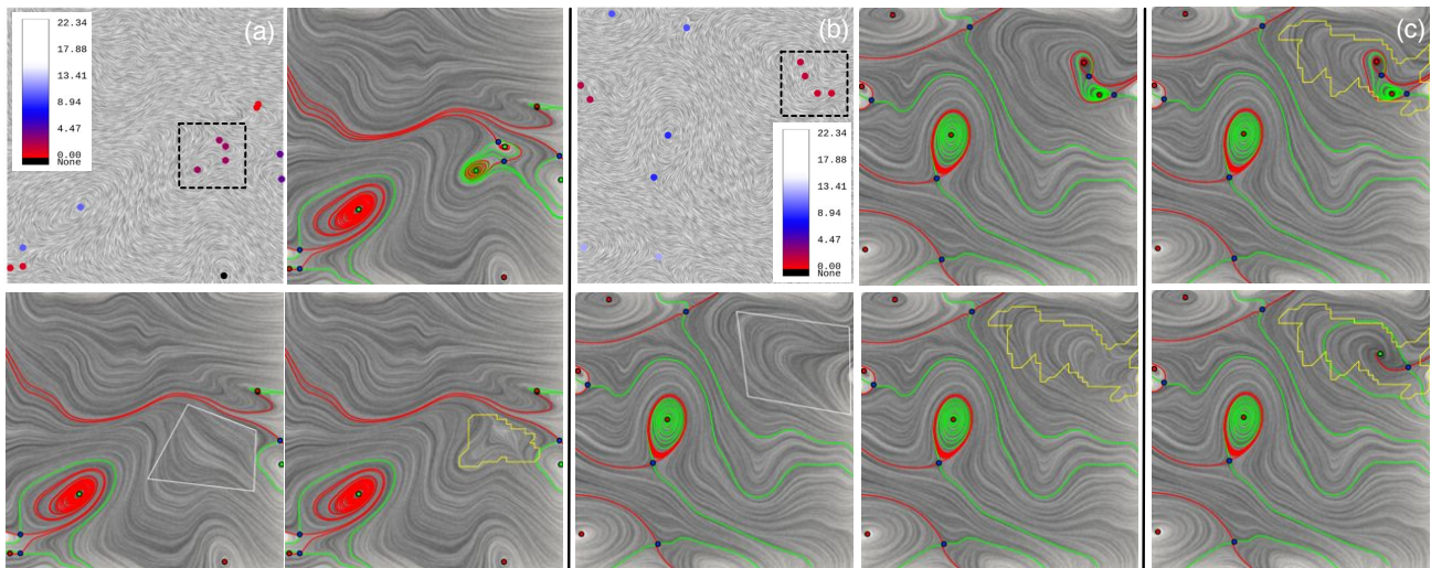
Fig. 12. The OceanA dataset: (a) #20311; (b)-(c) #21217. (a)-(b) For each subfigure, Top Row: Left – shows robustness values with region of interest highlighted; Right – shows the vector field marked by critical point types and its topological skeleton. Bottom Row: results after distance-based (left) and robustness-based simplifications (right). (c) A region (yellow boundary) with a nontrivial Conley index and uncovered boundary (top), where smoothing does not remove its critical points (bottom).
