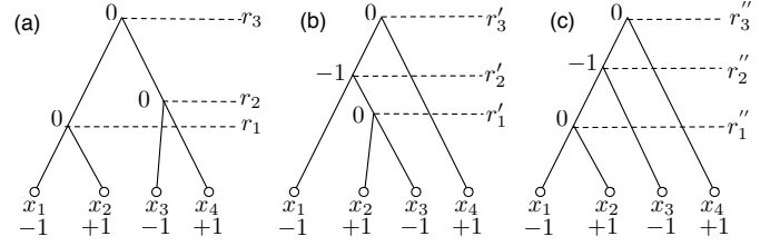
Fig. 18. Examples of two pairing switches between adjacent time slices. (a)-(c) t = i , t = i + 1 and t = i + 2 respectively.
