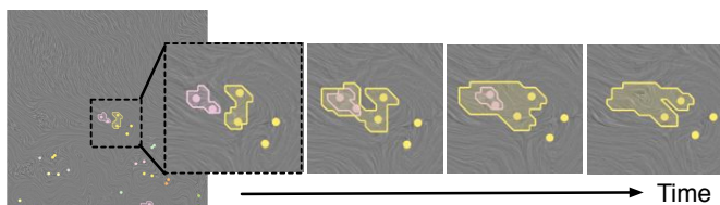
Fig. 19. Simplified critical points trajectories that intersect with one another. Time-varying simplification of SouthAtlantic.
