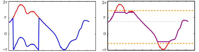
Fig. 10. SyntheticC. Left: The phase plot, original version (blue), and the phase-unwrapped version (red). Right: The phase plot with optimal unwrap point (orange) and the modified phase plot with boundary uncovered (purple).
