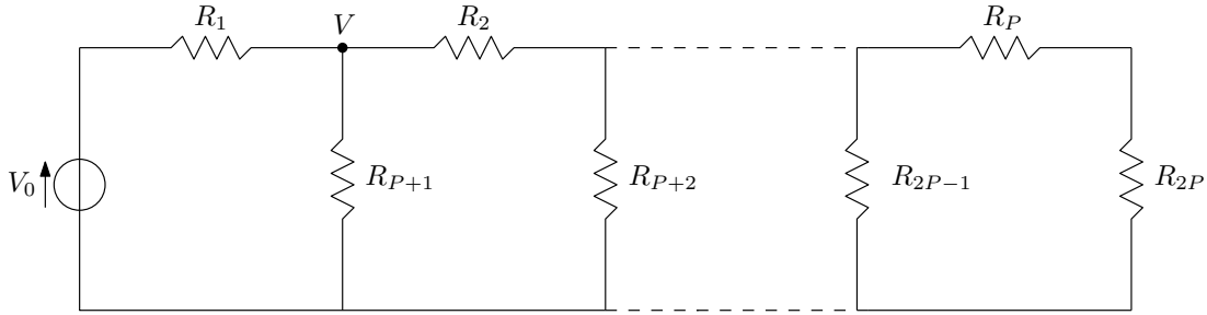
Figure 11. Resistor network
