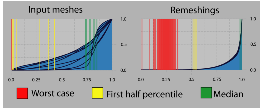
Figure 9: Cumulative histograms of incircle to circumcircle ratios. The histogram is normalized so that the best ratio is 1.0. The left column shows all the input meshes used in the paper, and the column in the right shows the results of all remeshes shown in this paper (80 in total).
