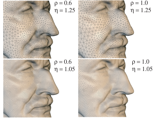
Figure 8: The effects of \rho and \eta on the resulting mesh. \rho controls the approximation accuracy: a bigger \rho will result in a coarser triangulation. \eta controls triangle grading: a larger \eta will result in more adaptive triangulations.
