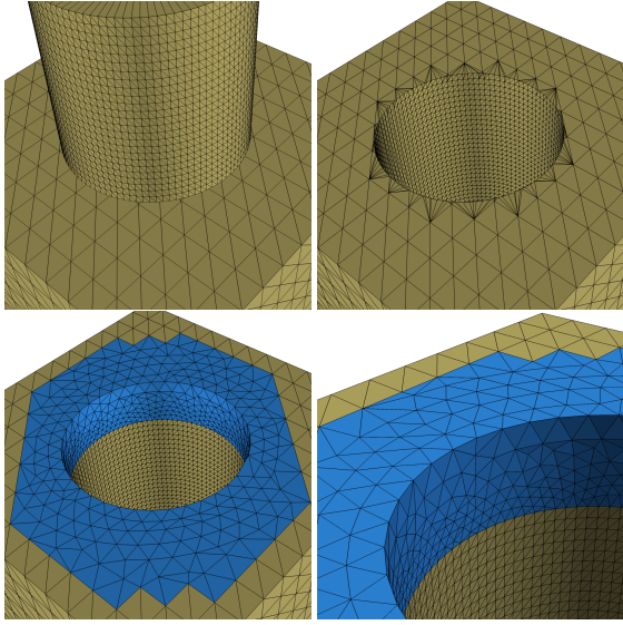
Figure 7: An example of a CSG difference operation. The output generated by Maya is shown in the upper-right corner, while the bottom row shows our operation. The algorithm only changes the portion shown in blue.
