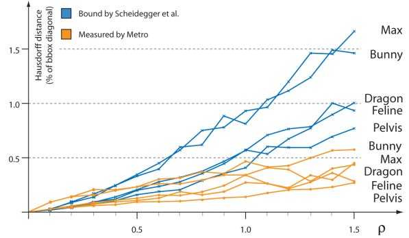
Figure 10: Predicted error and measured error, in percent of the bounding box diagonal.
