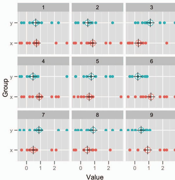
Fig. 3. A visual t -test. For each data set, the observations are shown as points and the group means as crosses. The accused is hidden amongst eight innocents. Can you spot him?
