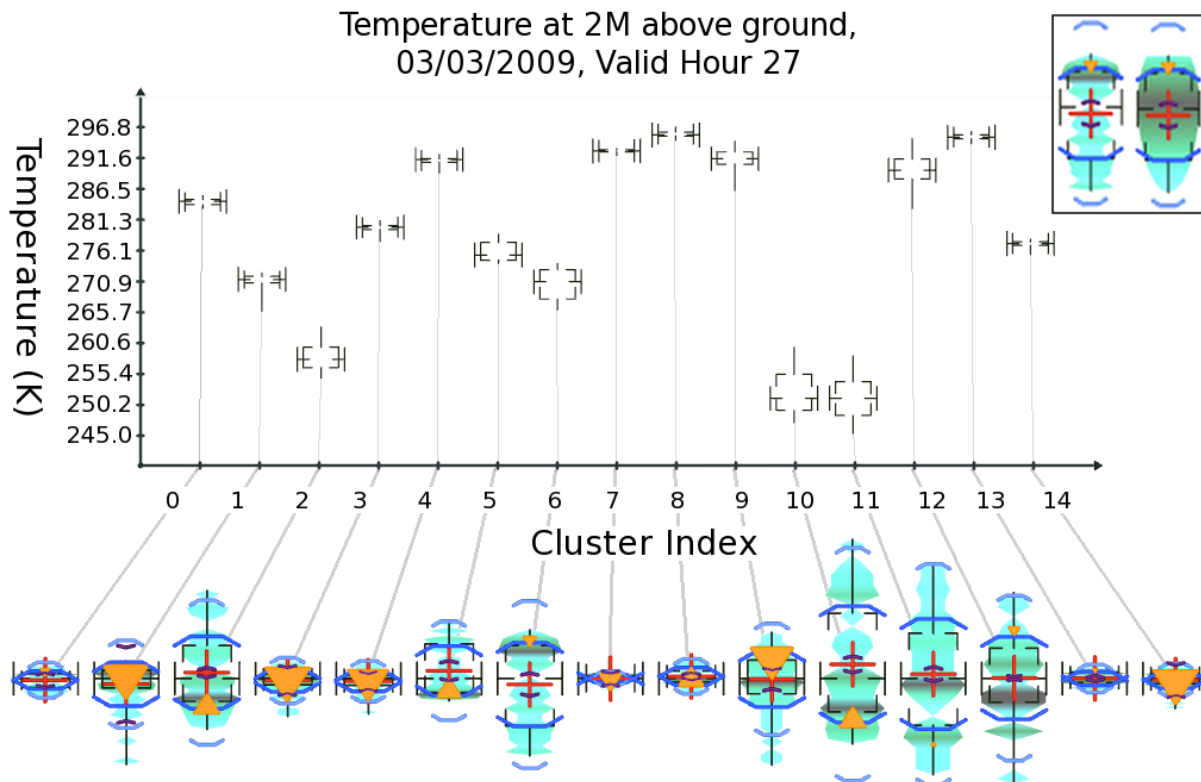
Figure 10: Summary plots for the points resulting from the clustering algorithm. Inset: (left to right) Histogram density estimation using 20 bins, and kernel density estimation.
