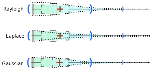
Figure 6: The results of fitting 3 canonical distributions to a single data set are shown as dotted lines on either side of the plot.
