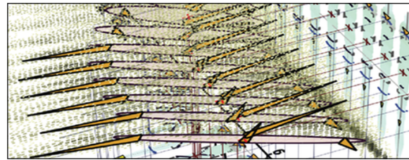
Figure 8: Close-up of the joint summary plot for multiple categorical datasets. While the joint histogram display induces some visual clutter, the cloud-like nature of the display gives a general feel of the density trend across the data. The covariance and skew variance glyphs help distinguish between each joint summary plot.
