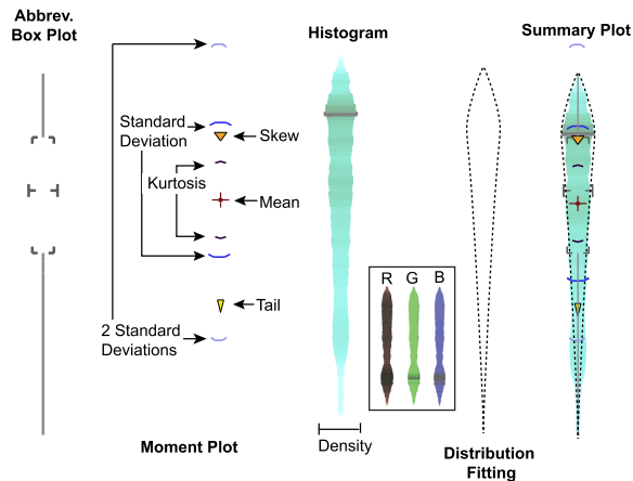
Figure 2: Anatomy of the summary plot. The abbreviated box plot displays the range of the data distribution. The moment plot shows higher order moments which describe feature characteristics. The histogram estimates the density of the distribution and is displayed using a symmetric display and a redundant colormap. Distribution fitting allows the user to compare the data against well-known distributions.
