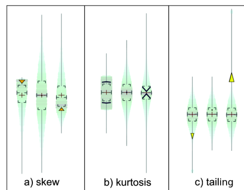
Figure 5: Glyphs for the higher-order central moments. Each triplet of distributions shows negative, close to zero, and positive values for the respective moment. Each higher-order moment is relative to the moments of a Gaussian distribution, which is the central distribution in each set.
