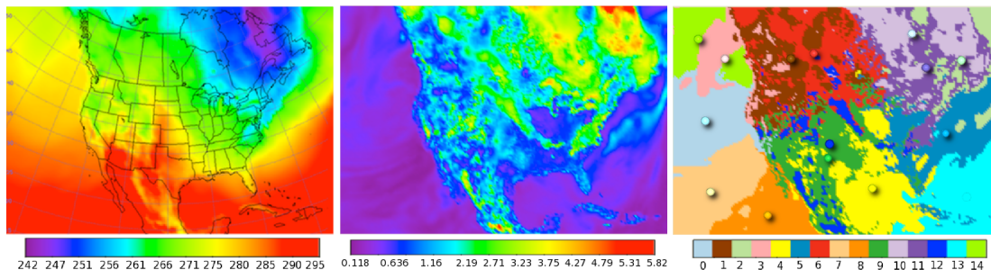
Figure 9: Temperature at 2M above ground at valid forecast hour 27. Color refers to the mean (leftmost) and standard deviation (center) of ensemble computed at each grid point. Results of k-medoids clustering algorithm [Bis06] on the temperature data (right). The domain is colormapped based cluster membership.
