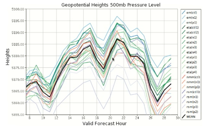
Fig. 8. Plume trend charts. These charts show the average of each ensemble model within a user-selected region of interest. Each model type is color-coded. The thick black line shows the mean across the entire ensemble.
