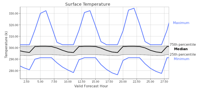
Fig. 7. Quartile trend charts. These charts show the quartile range of the ensemble within a user-selected region. Minimum and maximum are shown in blue, the gray band shows the 25th and 75th percentiles, and the median is indicated by the thick black line.
