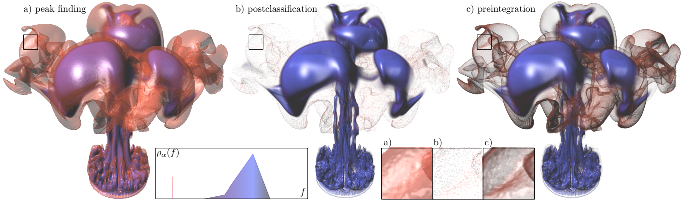
Fig. 3. Simulated temperature of a heptane fire, with a transfer function consisting of a near-Dirac peak (width \Delta f < 1e-4 ) in red, and a smoother feature for contrast in blue. Peak finding, postclassification and preintegration render at 7.1, 11.6 and 8.8 fps, respectively, at 1024x900.
