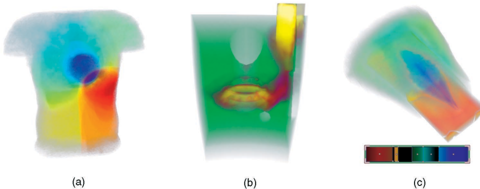
Fig. 7. Results of rendering the (a) torso, (b) spx, and (c) kew data sets with the HAVS algorithm.
