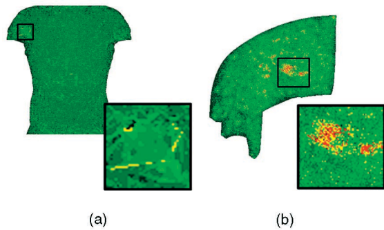
Fig. 6. Distribution of k requirements for the (a) torso and (b) spx2 data sets. Regions denote k size required to obtain a correct visibility sorting, for k > 6 (red), 2 < k \leq 6 (yellow), and k \leq 2 (green).
