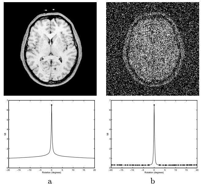
Fig. 2. Spatial correlation of image intensity values increases MI registration robustness. Top: a) original 256 \times 256 2-D MR image; b) image of a) shuffled by swapping 30,000 randomly selected pixel pairs. Both images have the same image content. Bottom: MI registration traces obtained using PV interpolation for in-plane rotation of each image over itself. Local maxima are marked with '*’.
