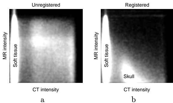
Fig. 1. Joint histogram of the overlapping volume of the CT and MR brain images of dataset A in tables II and III: a) initial position: I(CT, MR) = 0.46 ; b) registered position: I(CT, MR) = 0.89 . Misregistration was about 20 mm and 10 degrees (see the parameters in table III).
