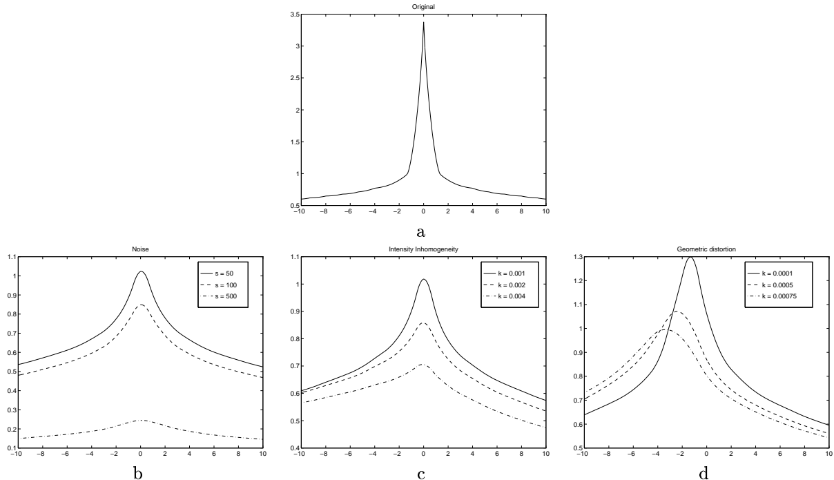
Fig. 9. MI traces using PV interpolation for translation in the x direction of the original MR image of dataset D over its degraded version in the range from -10 to +10 mm : a) original; b) noise; c) intensity inhomogeneity; d) geometric distortion.
