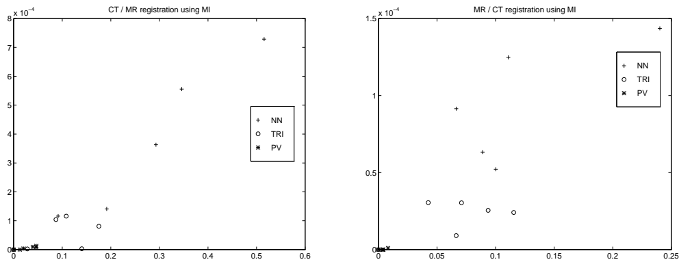
Fig. 5. Evaluation of the MI registration robustness for dataset A. Horizontal axis: norm of the difference vector |\alpha - \alpha^*| for different optimization strategies, using nearest neighbour (NN), trilinear (TRI) and partial volume (PV) interpolation. \alpha^* corresponds to the registration solution with the best value for the registration criterion for each of the interpolation schemes applied. Vertical axis: difference in the registration criterion between each solution and the optimal one. Left: using the CT image as the floating image. Right: using the MR image as the floating image.
