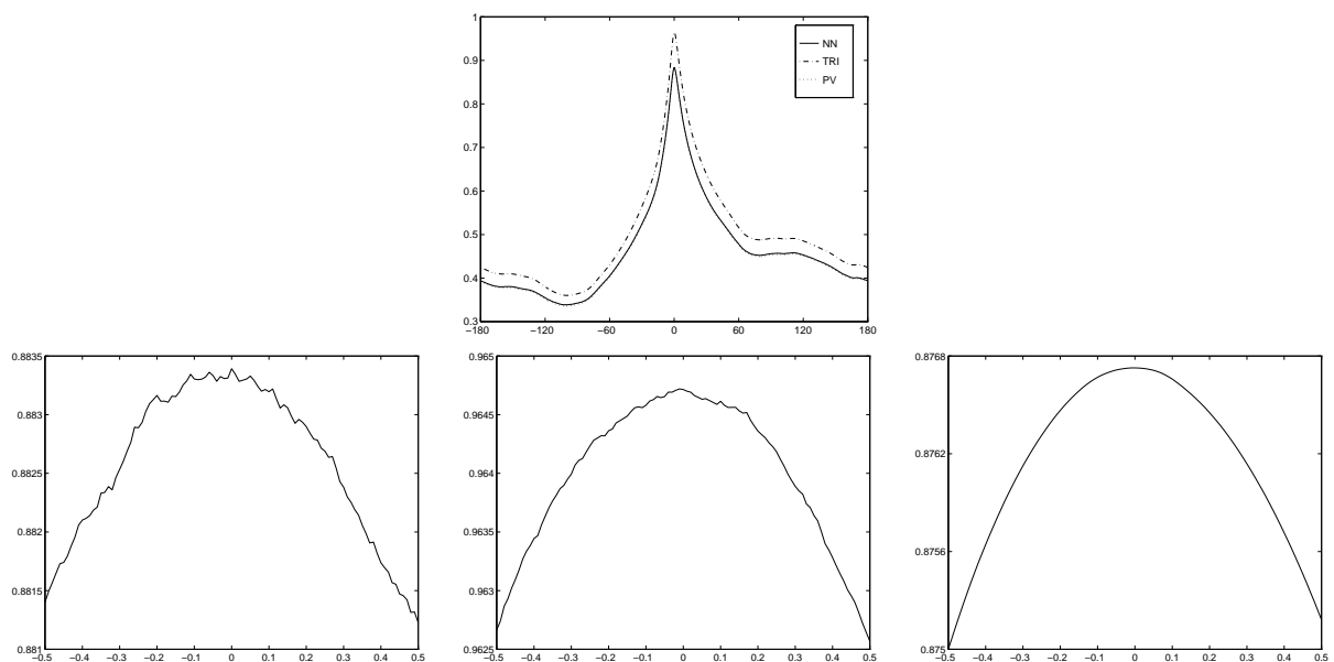
Fig. 6. MI traces around the optimal registration position for dataset A: rotation around the x axis in the range from -180 to +180 degrees (top) and from -0.5 to +0.5 degrees (bottom), using NN (left), TRI (middle) and PV (right) interpolation.
