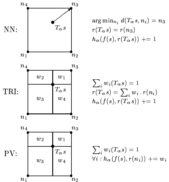
Fig. 3. Graphical illustration of NN, TRI and PV interpolation in 2-D. NN and TRI interpolation find the reference image intensity value at position T_\alpha s and update the corresponding joint histogram entry, while PV interpolation distributes the contribution of this sample over multiple histogram entries defined by its nearest neighbour intensities, using the same weights as for TRI interpolation.
