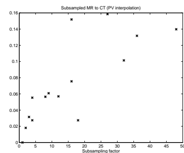
Fig. 7. Effect of subsampling the MR floating image of dataset A on the registration solution. Horizontal axis: subsampling factor f , indicating that only 1 out of f voxels was considered when evaluating the MI criterion. Vertical axis: norm of the difference vector |\alpha - \alpha^*| . \alpha^* corresponds to the registration solution obtained when no subsampling is applied.
