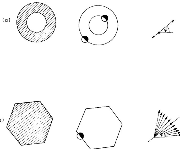
Fig. 7. Simple examples using R -tables; (a) washers; (b) hexagons.
