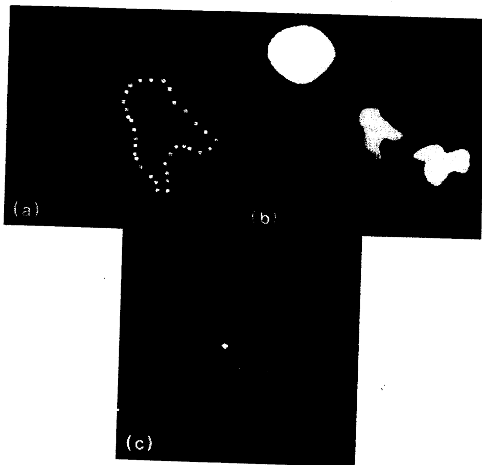
Fig. 8. An example. (a) Points on a shape used to encode R -table. (b) Image containing shape. (c) A plane through the accumulator array A(x, y, S_0, \theta_0) , where S_0 and \theta_0 are appropriate for the shape in the image ( S_0 = 64, \theta_0 = 0 ).
