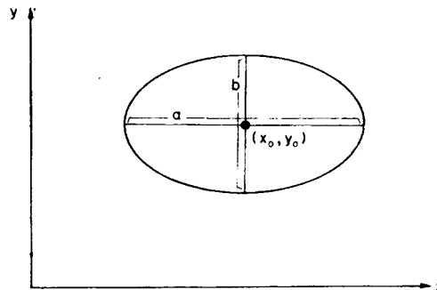
Fig. 4. Parametrization of an ellipse with major axis parallel to x -axis.
