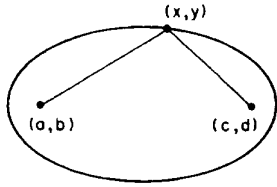
Fig. A1. String-tied-at-both-ends parameterization of an ellipse.
