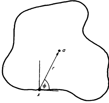
Fig. 6. Geometry for generalized Hough transform.
