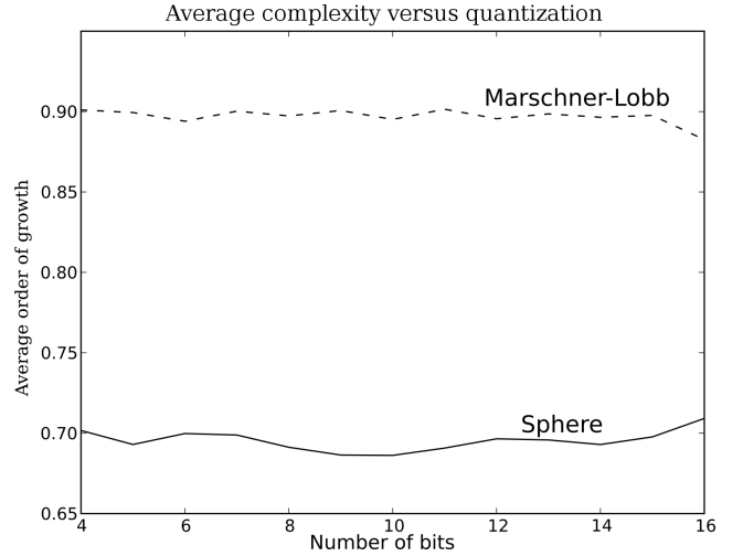
Fig. 9: Quantization level versus average complexity, with no noise. Quantization does not seem to influence the order of growth in either direction.
