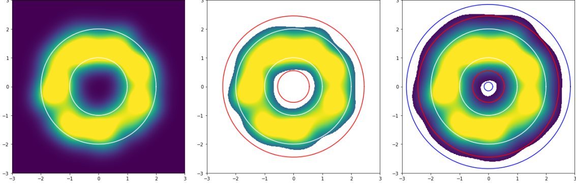
Figure 3: An example of the concentrated definition. The left side of the figure illustrates a probability density function (PDF) p which is \varepsilon -concentrated on an annulus \mathbb{X} . The center image illustrates the thickened space \mathbb{X}_\delta , bounded by the red curves, and the super-level set D_{L_1} . The right side of the figure illustrates the thickened space \mathbb{X}_\varepsilon , bounded by the blue curves, and the super-level set D_{L_2} . Together, we see that \mathbb{X} \subset D_{L_1} \subset \mathbb{X}_\delta \subset D_{L_2} \subset \mathbb{X}_\varepsilon .
