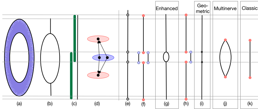
Figure 5: Variations of mapper graphs for the height function on a torus. (a) Torus with a height function. (b) Reeb graph. (c) Nice cover. (d) Visualization of the mapper cosheaf. (e) Stratification of \mathbb{R} . (f) Disjoint union of closed intervals, \tilde{\mathfrak{D}}(\mathcal{M}_{\mathcal{U}}(\mathcal{R}_f)) , with quotient isomorphic to the enhanced mapper graph. (g) Enhanced mapper graph, \mathfrak{D}(\mathcal{M}_{\mathcal{U}}(\mathcal{R}_f)) . (h) Disjoint union of closed intervals used to construct geometric mapper graph [35]. (i) Geometric mapper graph. (j) Multinerve mapper graph. (k) Classic mapper graph.
