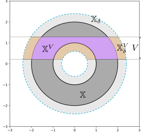
Figure 2: This figure illustrates the inverse images \mathbb{X}^V (in purple) and \mathbb{X}_\delta^V (union of tan and purple) for an annulus with height function and open interval V . Notice that in this example the \delta -thickening of \mathbb{X}^V would include \mathbb{X}_\delta^V as a proper subset, hence (\mathbb{X}^V)_\delta \neq \mathbb{X}_\delta^V .
