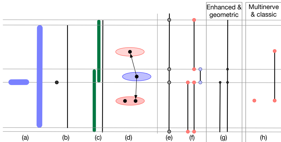
Figure 7: Variations of mapper graphs of a height function on a topological space consisting of two line segments. (a) A topological space consisting of two line segments. (b) Reeb graph. (c) Nice cover. (d) Visualization of the mapper cosheaf. (e) Stratification of \mathbb{R} . (f) Disjoint union of closed intervals with quotient isomorphic to the enhanced mapper graph. (g) Enhanced and geometric mapper graph. (h) Multinerve and classic mapper graph.
