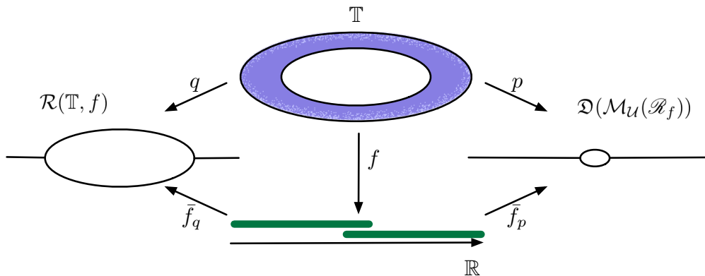
Figure 4: An example of the enhanced mapper graph \mathfrak{D}(\mathcal{M}_{\mathcal{U}}(\mathcal{R}_f)) and the Reeb graph \mathcal{R}(\mathbb{T}, f) of the height function f on the torus \mathbb{T} , with an open cover \mathcal{U} of f(\mathbb{T}) consisting of two open intervals. The maps q and \bar{f}_q are the natural quotient factorization of f obtained from the definition of the Reeb graph. Similarly, p and \bar{f}_p are the quotient map and factorization of f obtained from the definition of the enhanced mapper graph.
