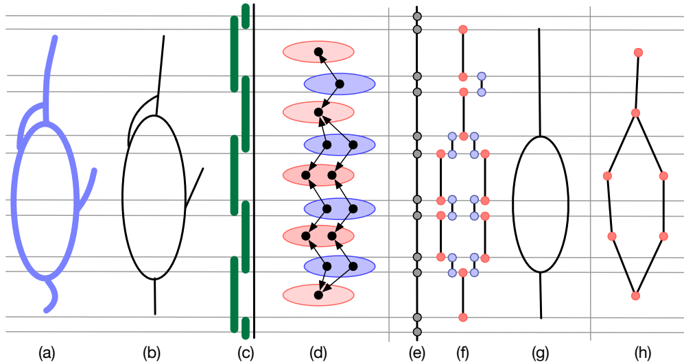
Figure 1: An example of an enhanced mapper graph. (a) An \mathbb{R} -space (\mathbb{X}, f) given by a topological space \mathbb{X} (in blue) equipped with a height function f : \mathbb{X} \rightarrow \mathbb{R} . (b) Reeb graph of (\mathbb{X}, f) . (c) Nice cover of \mathbb{R} with open intervals. (d) Visualization of the mapper cosheaf. (e) Stratification of \mathbb{R} . (f) Disjoint union of closed intervals (\tilde{\mathcal{D}} , in the notation of Section 2.3), with quotient isomorphic to the enhanced mapper graph. (g) Enhanced mapper graph (\mathcal{D} , in the notation of Section 2.3). (h) Classic mapper graph of (\mathbb{X}, f) .
