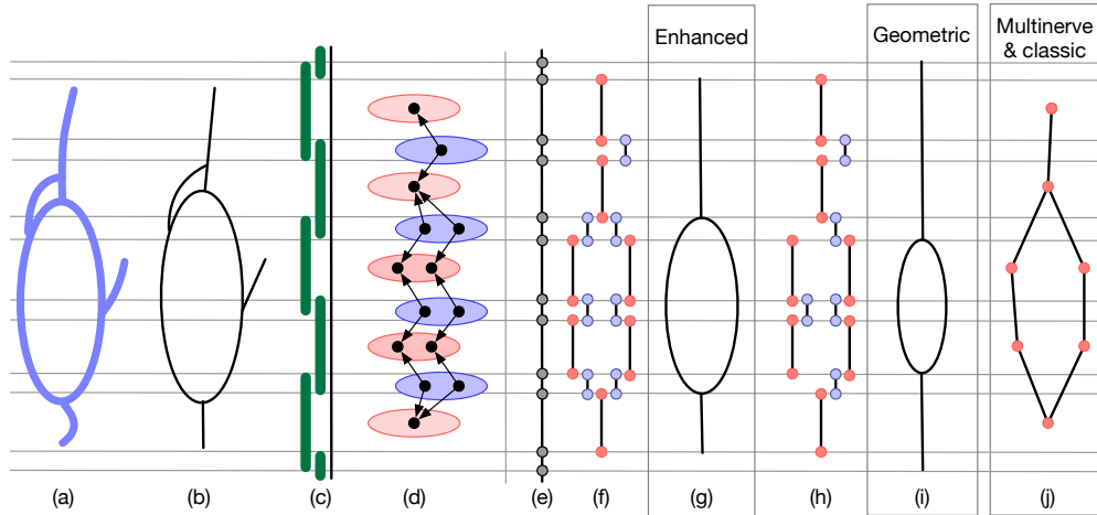
Figure 6: A return to the example illustrated in Figure 1. Variations of mapper graphs of a height function on a topological space. (a) A topological space with a height function. (b) Reeb graph. (c) Nice cover. (d) Visualization of the mapper cosheaf. (e) Stratification of \mathbb{R} . (f) Disjoint union of closed intervals with quotient isomorphic to the enhanced mapper graph. (g) Enhanced mapper graph. (h) Disjoint union of closed intervals used to construct geometric mapper graph [35]. (i) Geometric mapper graph. (j) Multinerve and classic mapper graph.
