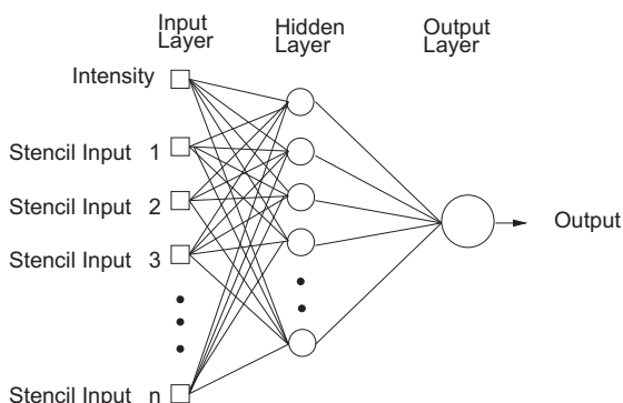
Fig. 2. Neural network diagram with one hidden layer. Inputs to the network include the image intensity and the values of the image at stencil locations.
