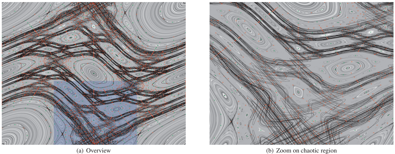
Fig. 7. Topology of the standard map for K=1.1 . At that stage the map exhibits sizable chaotic regions. However our algorithm is able to capture the most significant structures in the individual islands of the map. A very large numbers of fixed points are identified within the forming chaotic sea, which cannot be reliably linked to separatrices since the amplitude of chaotic motion is maximized along those separatrices. While these points appear random, note the many degrees of symmetry which they exhibit.
