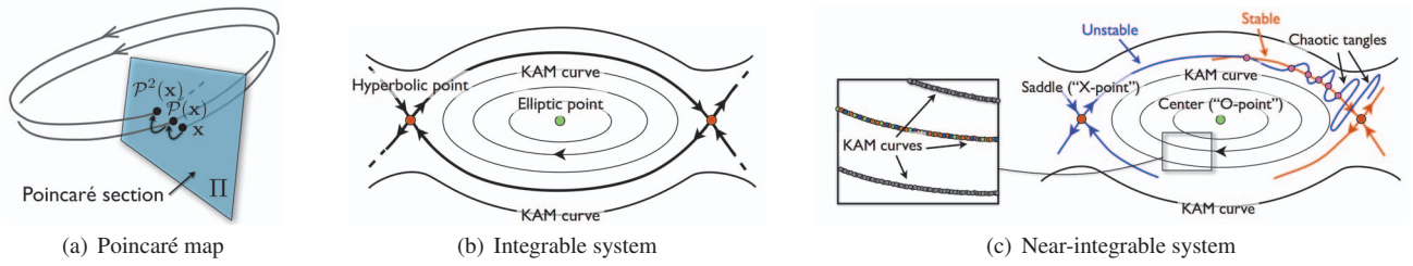
Fig. 2. (a) illustrates two iterations of a Poincaré map. (b) and (c) illustrate islands of resonance in the topology of the Poincaré section. In the integrable case (b), separatrices connect saddle points in the Poincaré map, forming the boundary of an island containing a center point. In the chaotic case (c), the connections are replaced by the intersection of stable and unstable manifolds at an infinite number of points, forming the tangles that characterize chaos. Quasi-periodic orbits exist both inside and outside of the island, where they densely populate KAM manifolds.
