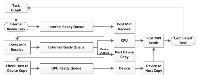
Figure 1: Uintah Multi-Queue Task Scheduling
