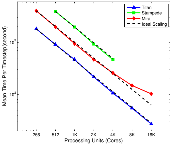
Figure 11: RMCRT Strong Scaling
