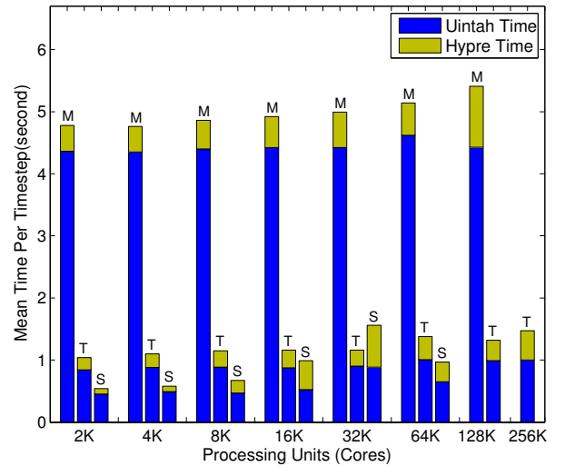
Figure 9: ARCHES with Hypr Weak Scaling
