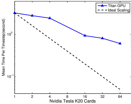
Figure 10: Single Level RMCRT Strong Scaling On Titan GPU
