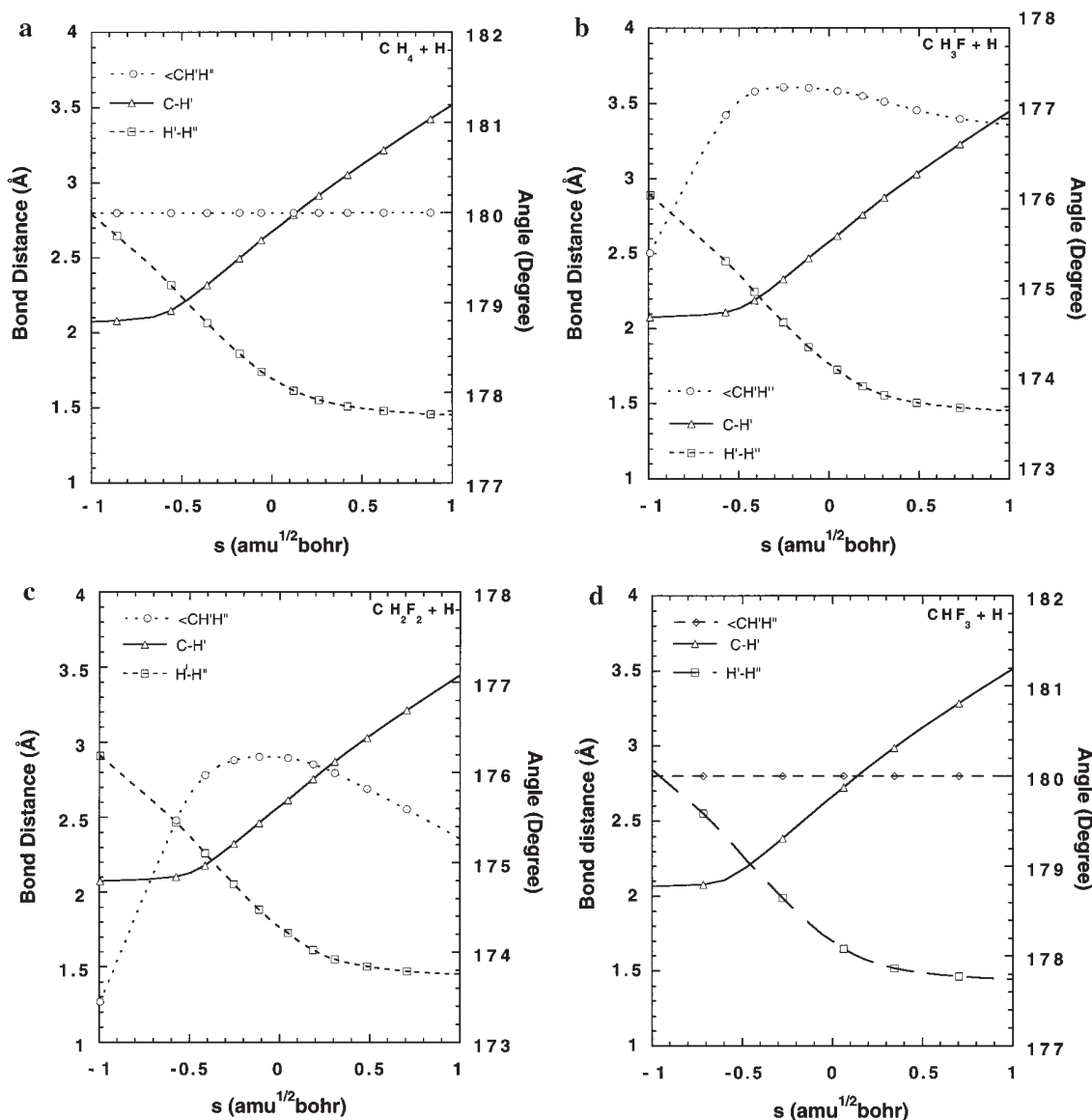
Figure 1. (a) Selected geometrical profiles along the B3LYP/cc-pVDZ minimum energy path for the \text{CH}_4 + \text{H} \leftrightarrow \text{CH}_3 + \text{H}_2 reaction plotted vs the reaction coordinate s in the mass weighted coordinates. (b) Same types of geometrical profiles as those in a for the \text{CH}_3\text{F} + \text{H} \leftrightarrow \text{CH}_2\text{F} + \text{H}_2 reaction. (c) Same types of geometrical profiles as those in a for the \text{CH}_2\text{F}_2 + \text{H} \leftrightarrow \text{CHF}_2 + \text{H}_2 reaction. (d) Same types of geometrical profiles as those in a for the \text{CHF}_3 + \text{H} \leftrightarrow \text{CF}_3 + \text{H}_2 reaction.
