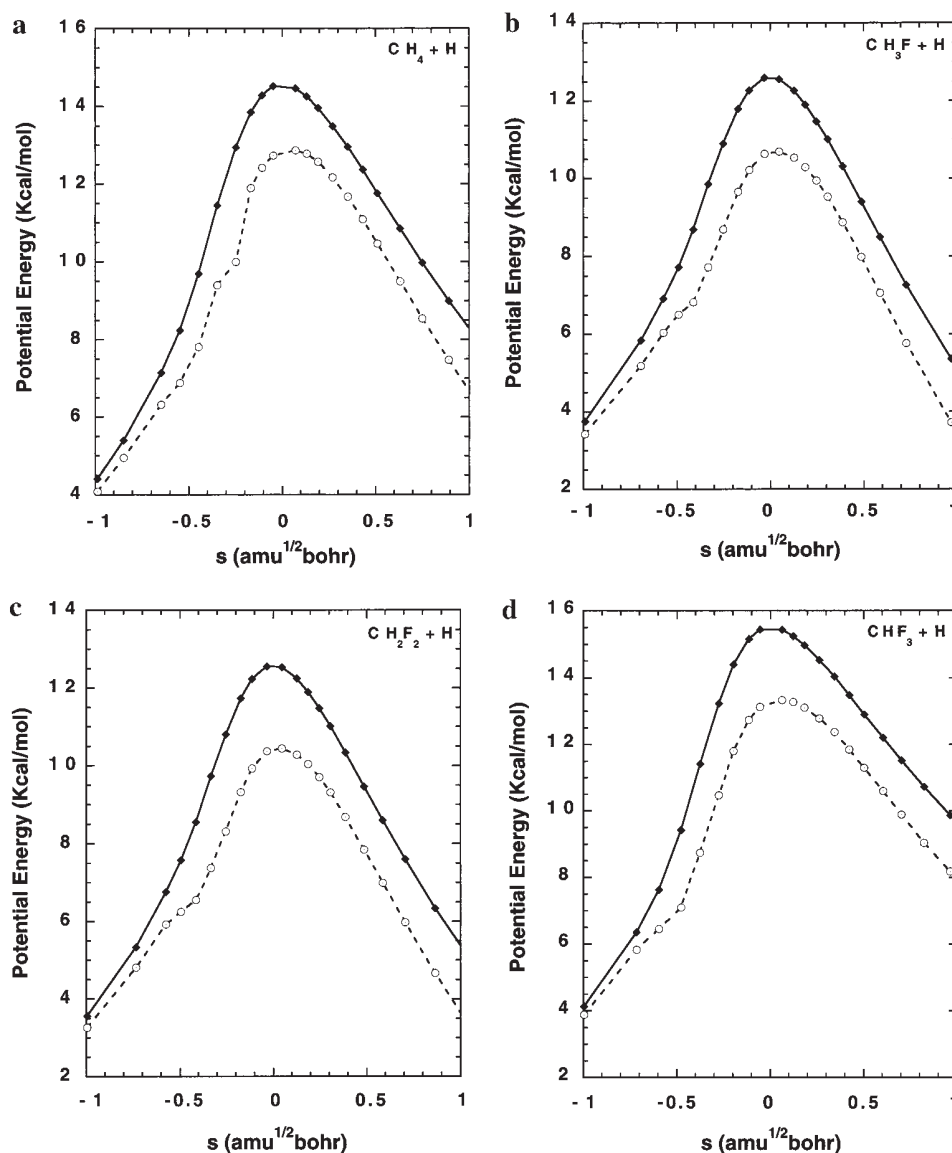
Figure 2. (a) The classical potential energy V_{\text{MEP}}(s) (solid line) and the vibrationally ground-state adiabatic potential energy V_{\text{a}}^{\text{G}}(s) (dashed line) curves along the B3LYP/cc-pVDZ minimum energy path for the \text{CH}_4 + \text{H} \leftrightarrow \text{CH}_3 + \text{H}_2 reaction plotted vs the reaction coordinate s . (b) Same types of curves as those in a for the \text{CH}_3\text{F} + \text{H} \leftrightarrow \text{CH}_2\text{F} + \text{H}_2 reaction. (c) Same types of curves as those in a for the \text{CH}_2\text{F}_2 + \text{H} \leftrightarrow \text{CHF}_2 + \text{H}_2 reaction. (d) Same types of curves as those in a for the \text{CHF}_3 + \text{H} \leftrightarrow \text{CF}_3 + \text{H}_2 reaction.
