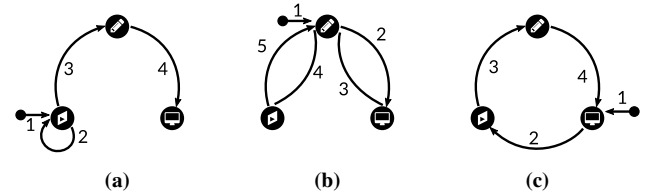
Figure 4: Three examples of transitions within the CLUE model, highlighting different entry points. Numbers indicate the order in which the stages are visited by the user.
