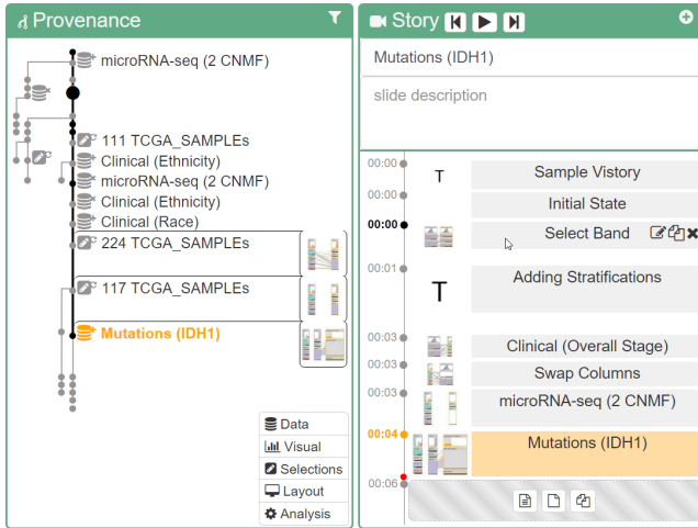
Figure 6: Close-ups of the provenance and story views. Based on the DoI, exploration states are represented at different levels of detail in the provenance view. The structure of the Vistory, shown on the right, corresponds to a path through the provenance graph, which is shown as a thick black line in the provenance visualization. Both the active slide in the story view and the associated exploration state in the provenance graph are highlighted in orange.
