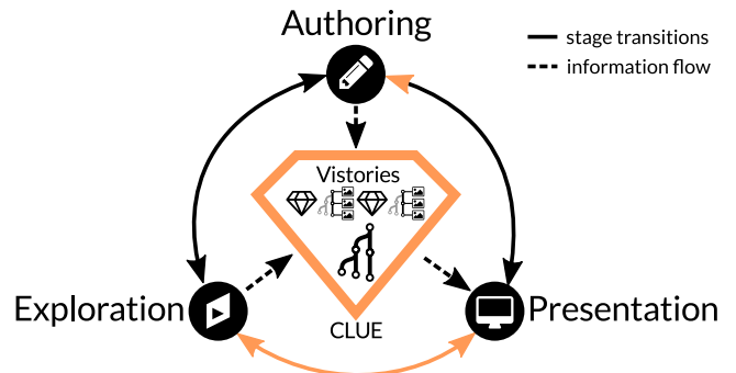
Figure 3: Information flow and stage transitions using the CLUE model. The provenance graph of an exploratory session and Vistories (interactive visual stories) are in the center. Solid edges indicate possible stage transitions, dashed lines indicate information flow. In the exploration stage, provenance data is generated; in the authoring stage a Vistory is created by curating provenance data, which is then used in the presentation stage. Note that consumers of a Vistory can also switch to any other stage.
