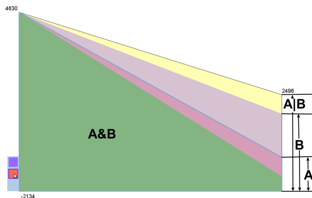
Figure 2: Two filters combined with logical OR, both sub-filters stacked over each other. The largest filter with the light yellow background is the resulting filter ( A|B ), the two purple filters are the combined sub-filters (just A or just B) and the green filter on top of all filters represents the intersection of the elements filtered by both sub-filters ( A\&B ).
