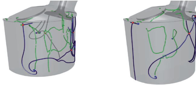
Fig. 7. Two frames from a time-varying visualization of tumble motion using a combination of cutting-plane topology (green lines) and boundary topology (blue lines). Where the critical point paths computed over the cutting-plane parameter range intersect the boundary, singularities appear there, too. This is a prime example of a hybrid approach being used to investigate the relationship between boundary and volume methods (colorplate on p. 215).
