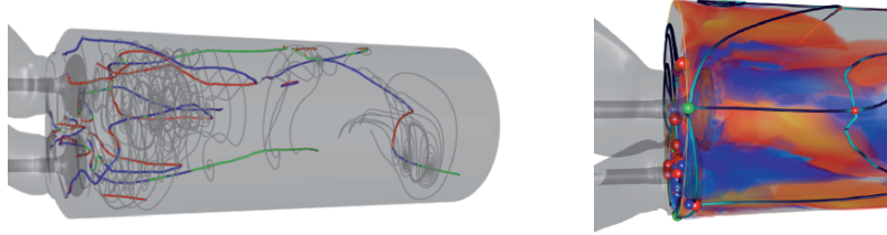
Fig. 4. Left: Cutting-plane topology applied to the diesel engine. Plane separatrices are colored gray. Despite the visual inexactness, swirl structures emerge clearly. Critical points paths are colored according to nature. It appears the overall swirl motion is fueled by several parallel vortices at the top of the cylinder. The main swirl motion core is disrupted near the middle. Right: Visualization of the rotational directions in the vortex system at the top of the diesel engine cylinder. The transfer function is identical to that of Fig. 6. The counter-rotating vortices appear in blue and in red depending on rotation direction. On the boundary, the topological analysis extracts and visualizes separation lines between individual vortices (color coding as in Figs. 2 and 3). (Colorplate on p. 214.)
