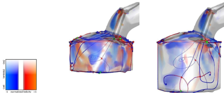
Fig. 6. Unsteady visualization of vortices from in-cylinder tumble motion in a gas engine and its relationship to the boundary. During the valve cycle (top left to bottom right), the piston head that shapes the bottom of the geometry moves down (not shown). The volume rendering shows vortices using a two-dimensional transfer function of \lambda_2 and normalized helicity (legend). The main tumble vortex is extracted and visible as off-center and with an undesired diagonal orientation. The flow structure on the boundary is visualized using boundary topology, with critical points colored according to their nature (cf. Fig. 2). A direct correspondence between the volume and boundary visualizations can be observed. In the third image, the intersection of the main vortex with the boundary results in critical points on the front and back walls.
