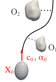
Fig. 1. Overview of geodesic regression with estimated parameters in red.
