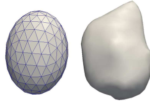
Fig. 2. Initial baseline shape and observed amygdala.
