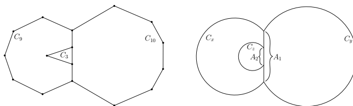
■ Figure 5 A finite vertex subset (left) and a metric graph (right) built by first gluing C_x to C_y along A_1 , and then gluing C_z to the result along A_2 .
