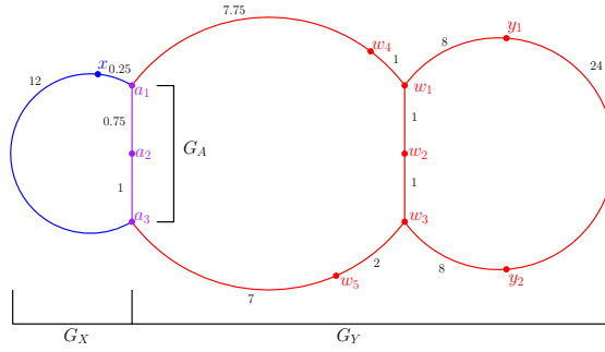
■ Figure 3 Two graphs, G_X (blue) and G_Y (red), glued along G_A (purple). Distances between points are denoted in black.
