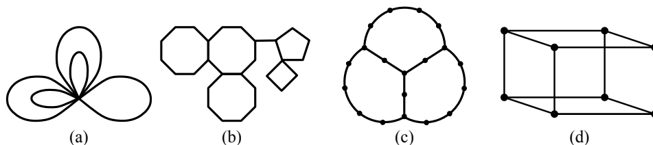
Figure 4 Graphs (a) and (b) can be characterized while (c) and (d) cannot.
