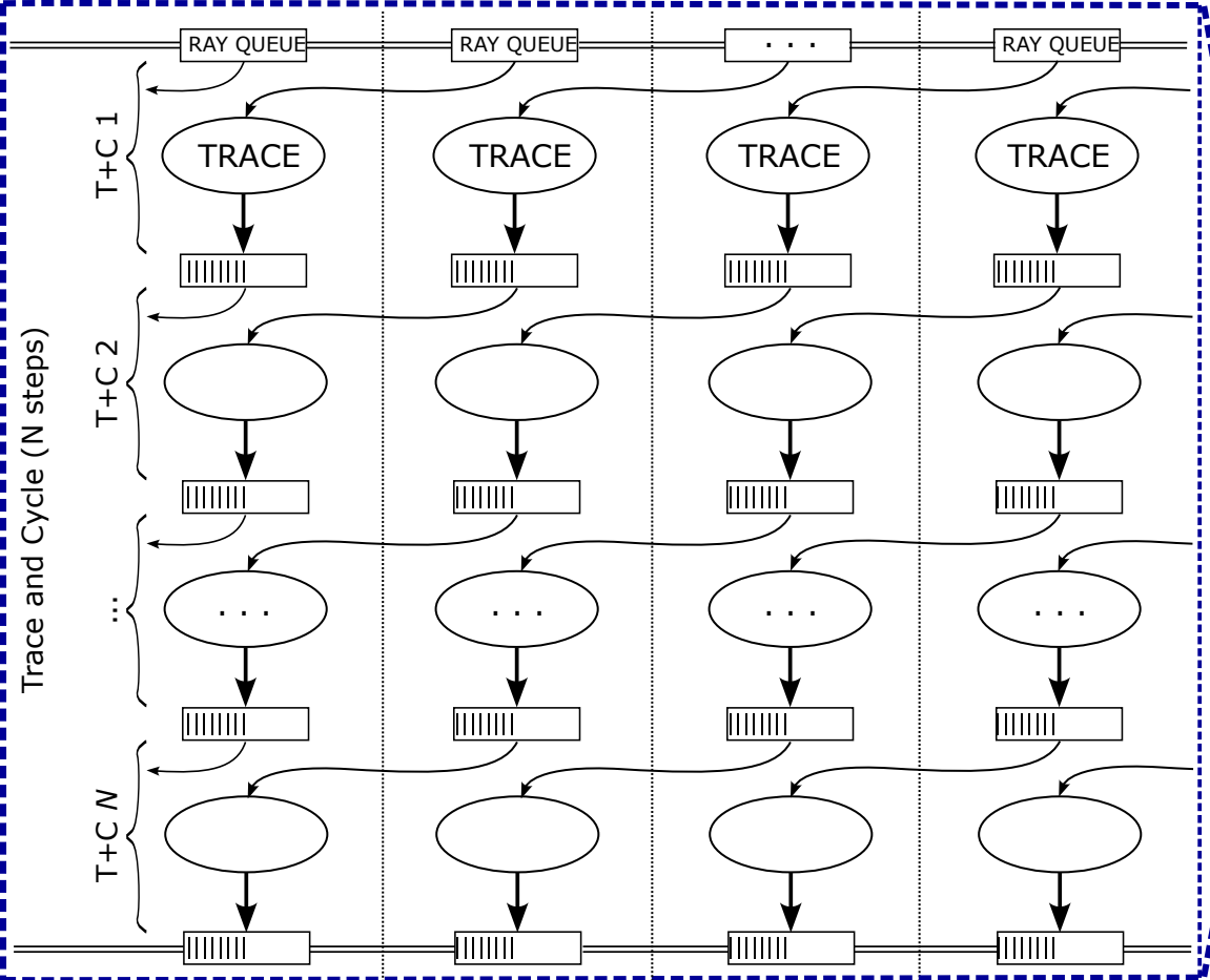
collaborative trace stage: N trace-and-cycle rounds
