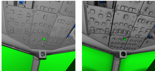
Figure 6: Comparison between Lambertian shading with shadows and ambient occlusion (5x5 filter, four secondary rays).
