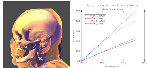
Figure 7: Scalability of Utah ray tracing engine: The graph on the right shows almost linear scaling behavior for up to 128 CPUs.
