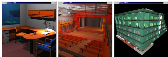
Figure 1: Interactive ray tracing: The office, conference and Soda Hall models contain roughly 40k, 680k, and 8 million triangles, respectively. Using a software ray tracing implementation running on a single PC (Dual Pentium-III, 800 MHz, 256MB) at a resolution of 512 2 pixels, these scenes render at roughly 3.6, 3.2, and 1.6 frames per second.
