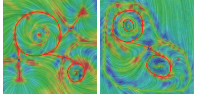
Fig. 11. This figure shows the density maps of the sample rates of the two analytic fields using our algorithm. The color coding of the density map uses red for the region with a larger sampling rate and blue for a lower sampling rate.
