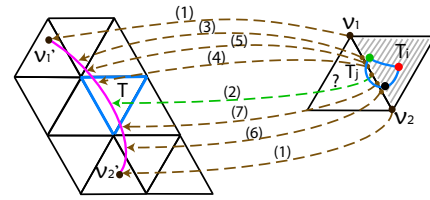
Fig. 10. This figure describes how the backward mapping and the adaptive edge sampling help to find the complete edges of the directed graph under a highly stretched flow. The edge (v_1, v_2) has been sampled to obtain the continuous triangle strip that contains the image of it using Algorithm 1. The brown dashed curves illustrate the backward tracing along -V . (1)–(7) indicate the sampling and tracing order. Note that step (2) gives rise to the edge T \rightarrow T_j that is missed in the case (7) of Figure 7.
